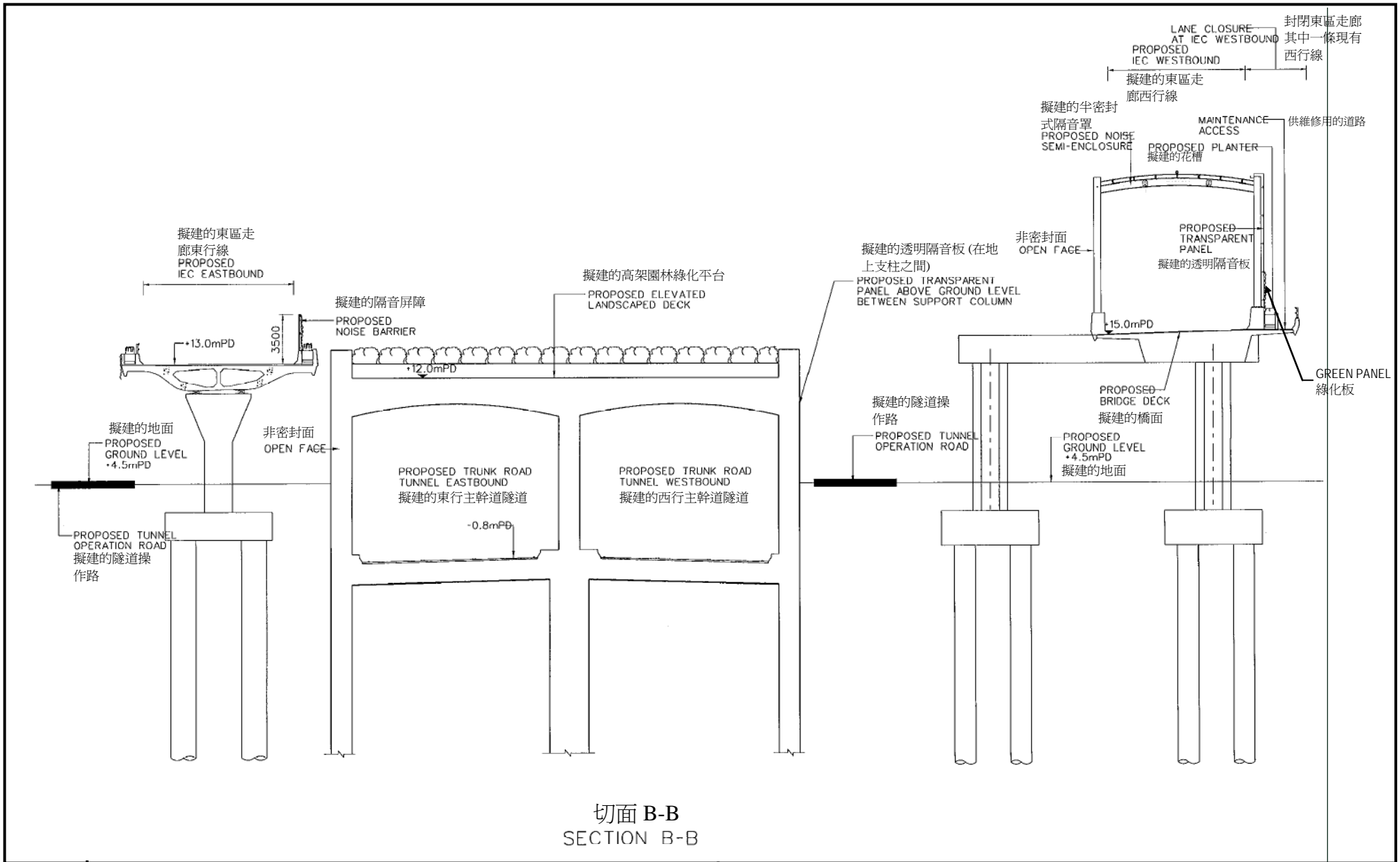
Figure 4e: Section of Direct Noise Mitigation Measures 圖 4e: 直接噪音緩解措施切面圖
